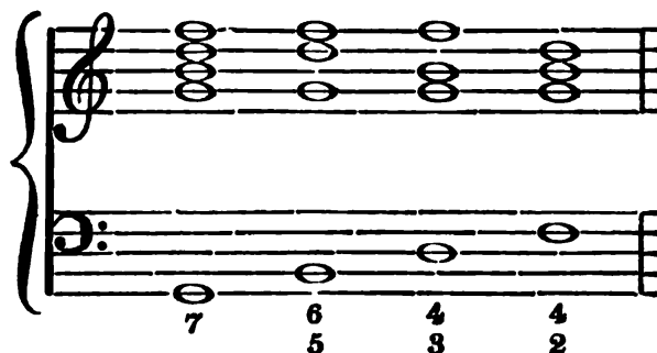
The 7th and its derivatives.
