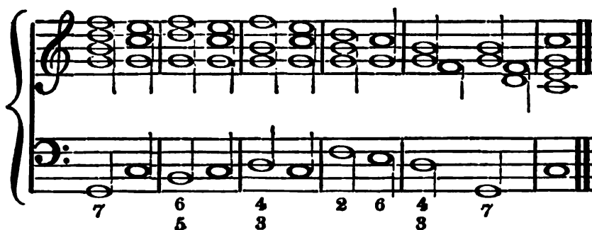
The 7th and its derivatives.
